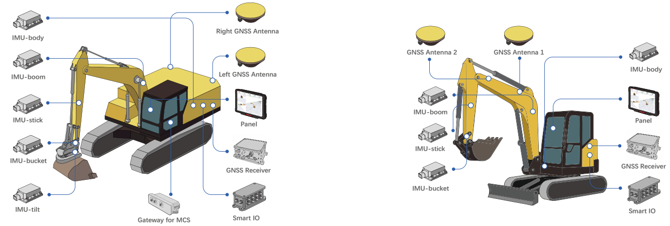
Standard Kit + Dual Boom Kit
